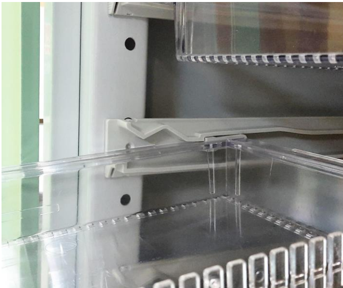
Position #1 (upper support) Tray slope \alpha angle: 50
